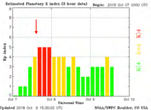
Figure 2 – Planetary K Indices
